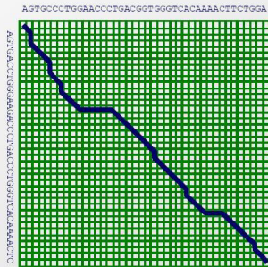
Global alignment
