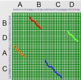
Local alignment
